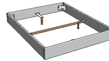
Crosstraver Quertraverse Traverse transversale Central cross bar
